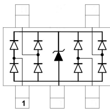
Circuit and Pin Schematic
